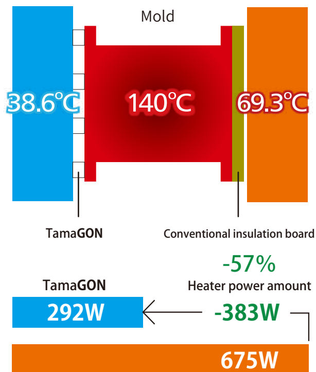
Insulation 'TamaGON' parts
